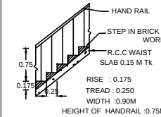
STAIR DETAILS
