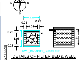
DETAILS OF FILTER BED & WELL
