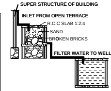
RAINWATER HARVESTING
