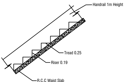
STAIR DETAILS
