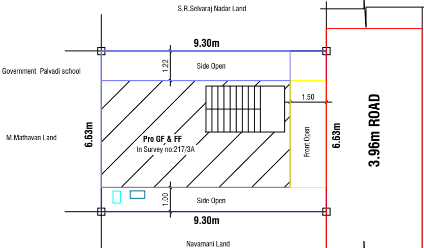
SITE PLAN (1:100)
