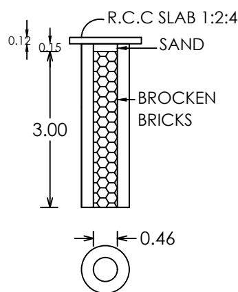
Percolation Pit
