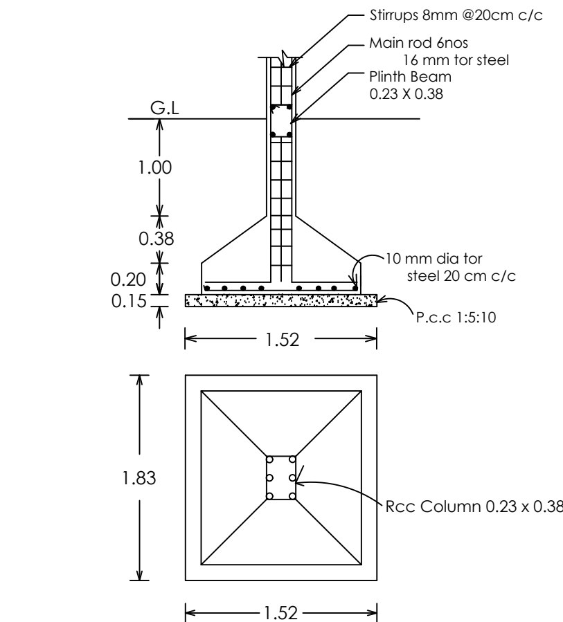
Details of column footing
