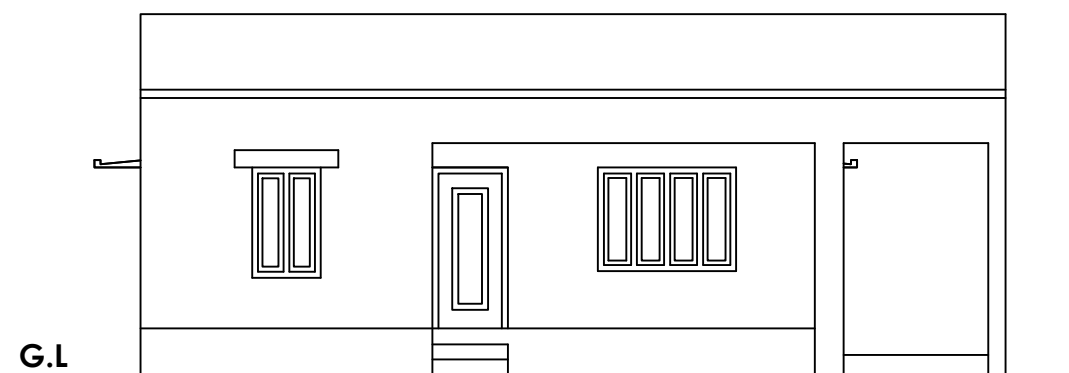
FRONT ELEVATION
