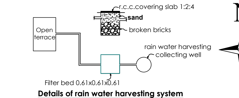
Details of rain water harvesting system
