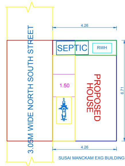
SITE PLAN
