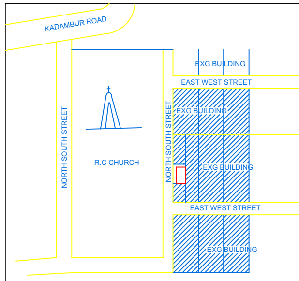
TOPO PLAN SCALE 1:500
