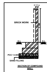
SECTION OF COMPOUND WALL
