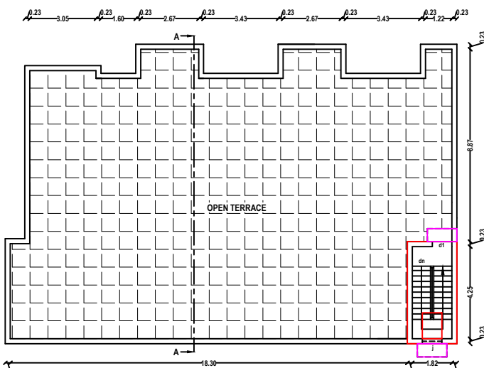
PROPOSED PLAN - HEAD ROOM (RESIDENCE)
