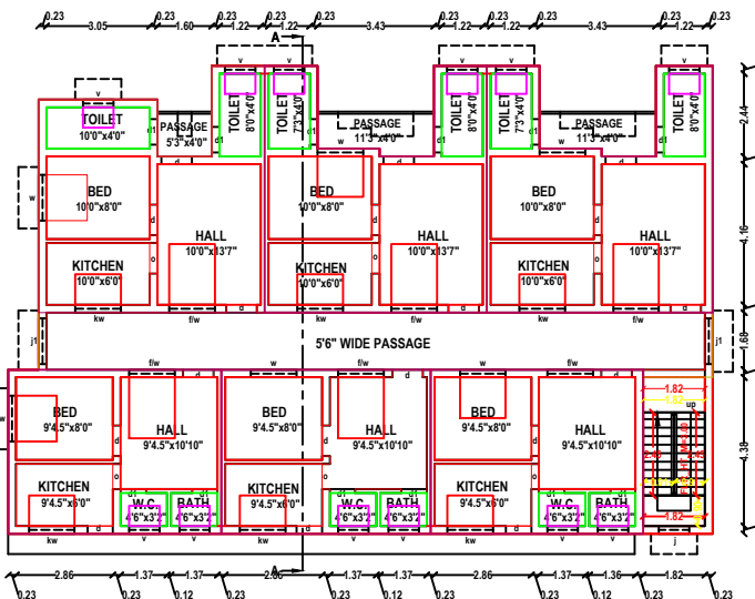
PROPOSED PLAN - FIRST FLOOR (RESIDENCE)
