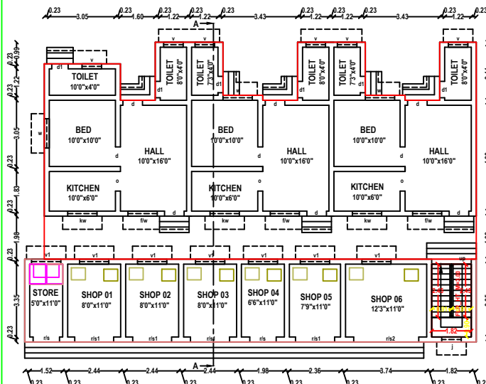
EXISTING PLAN - GROUND FLOOR (SHOP + RESIDENCE)
