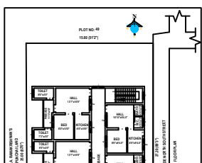
EXISTING PLAN - GROUND FLOOR (SHOP + RESIDENCE)
