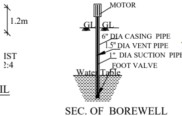
SEC. OF BOREWELL
