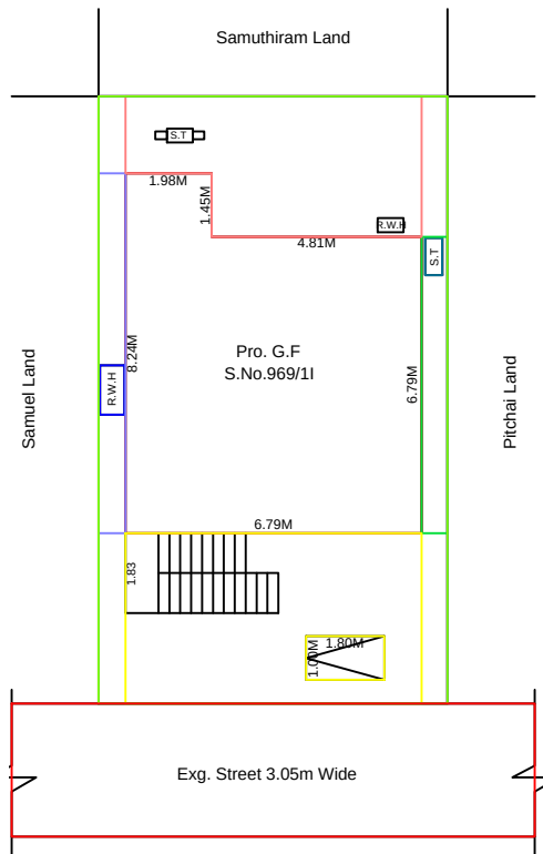
SITE PLAN
