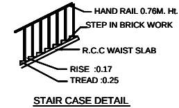
STAIR CASE DETAIL
