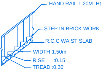
STAIR DETAIL
