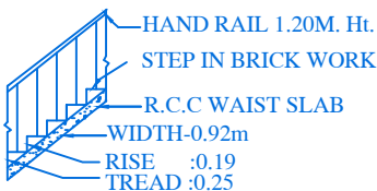
STAIR DETAIL
