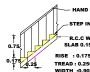
STAIR DETAILS
