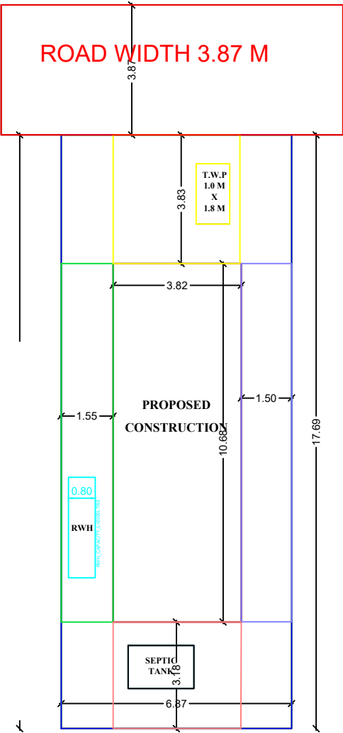
PERUMAL EXG HOUS SITE PLAN SCALE : 1"= 8' OR [1 : 100]
