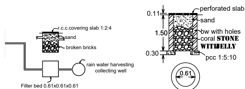
DETAILS OF RAIN WATER HARVESTING SYSTEM
