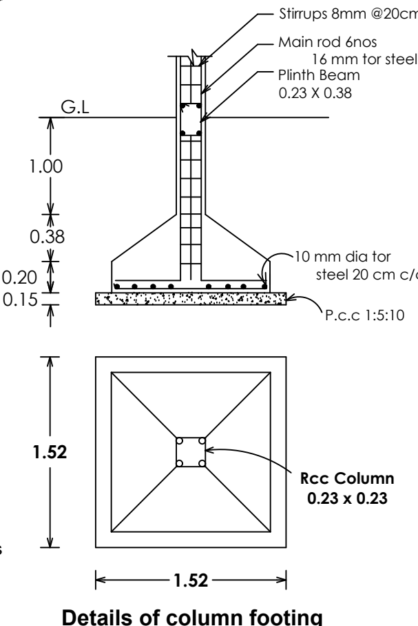
Details of column footing
