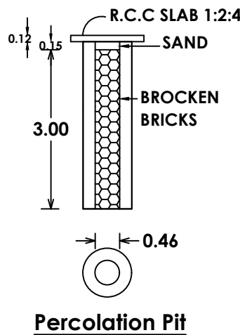
Percolation Pit
