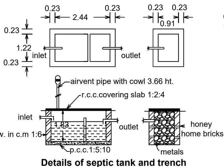
Details of septic tank and trench
