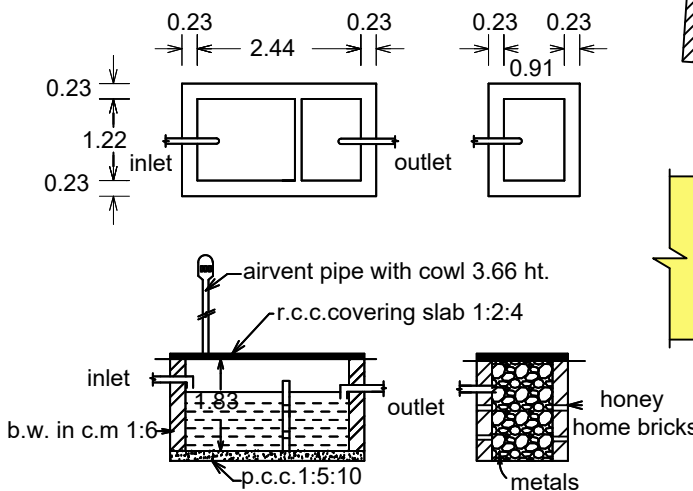
Details of septic tank and trench
