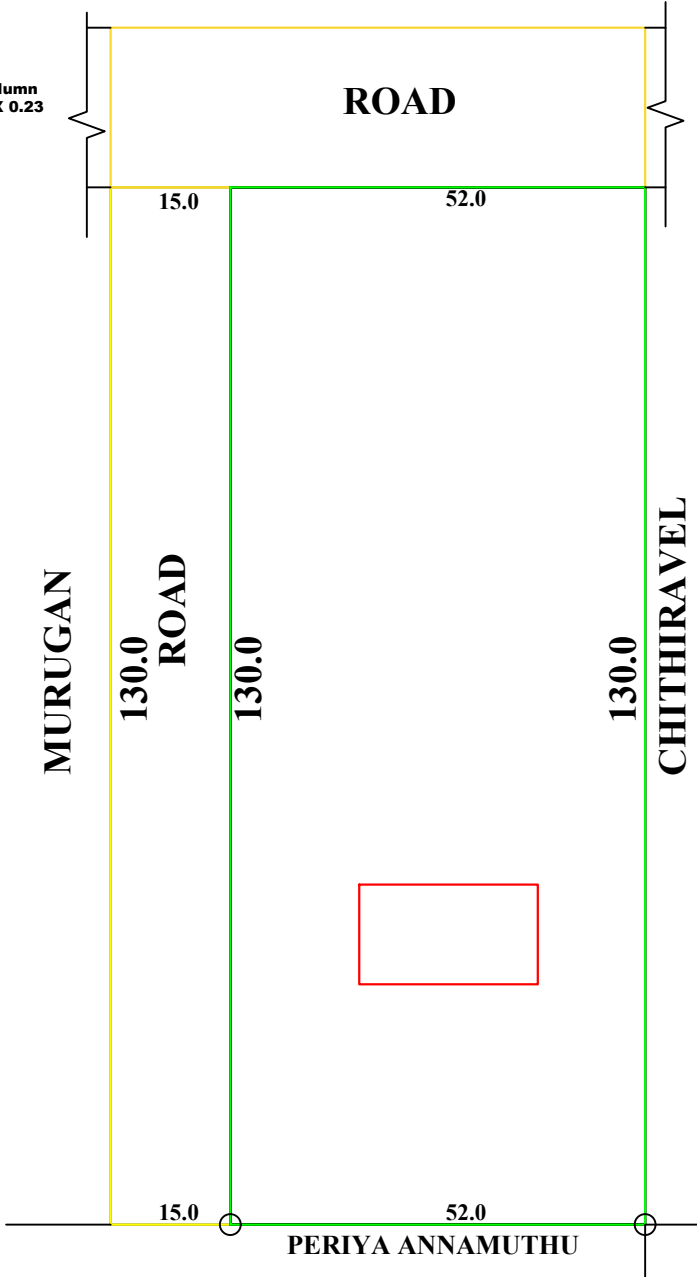
SITE PLAN
