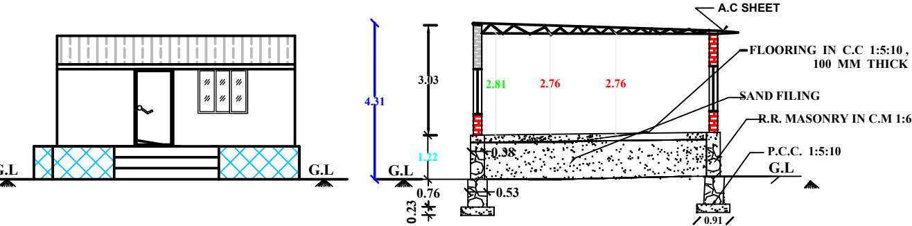
FRONT ELEVATION
