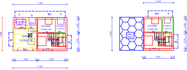
SHOP PLAN HOUSE PLAN HOUSE PLAN GROUND FLOOR PLAN FIRST FLOOR PLAN
