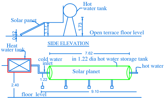
SOLAR WATER HEATER PLANT
