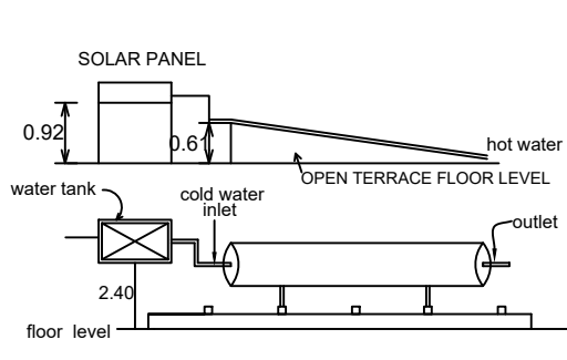
Details of solar water heating system
