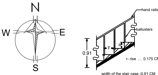
Details of staircase
