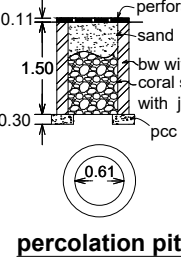
percolation pit
