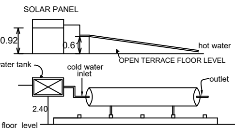
Details of solar water heating system
