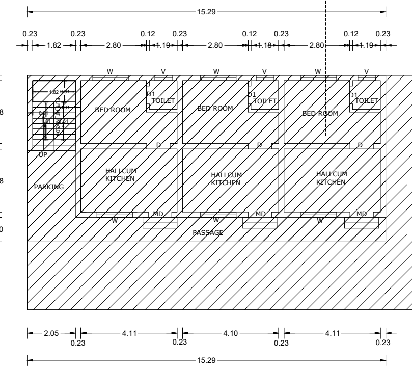
EXG. GROUND FLOOR PLAN
