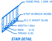
STAIR DETAIL
