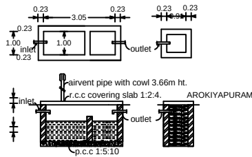
Details of septic tank & trench
