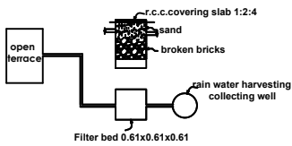
Details of rain water harvesting system
