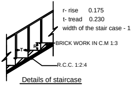
Details of staircase
