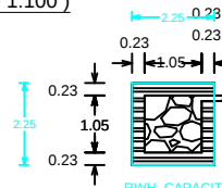
DETAILS OF FILTER BED & WELL
