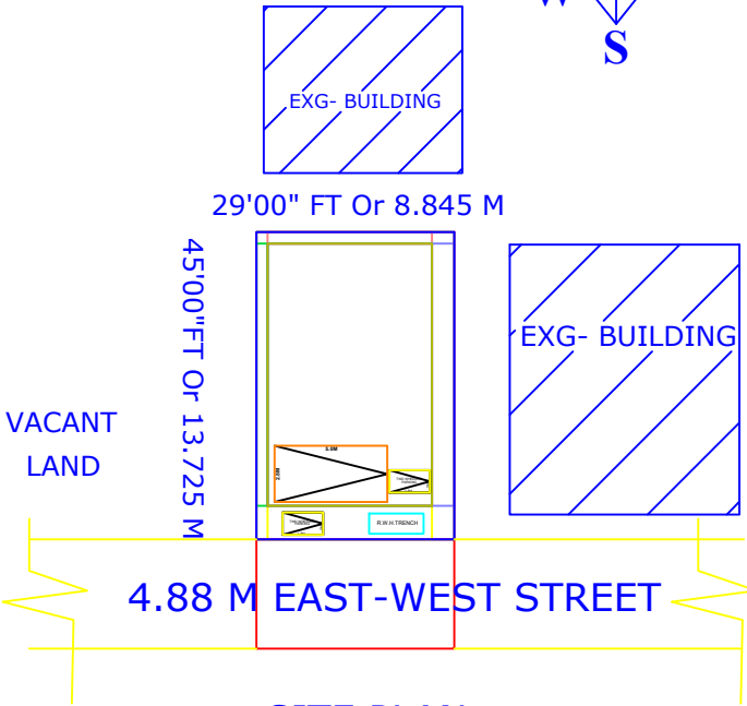
SITE PLAN
