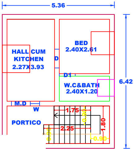
FLOOR PLAN
