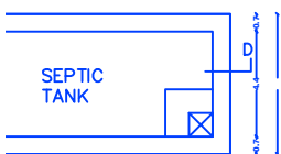
PLAN OF SEPTIC TANK SCALE 1"=2'-0"
