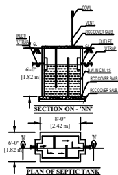
PLAN OF SEPTIC TANK
