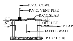
SEC. OF SEPTIC TANK
