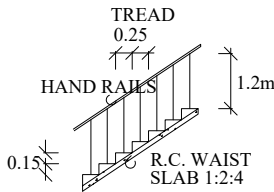
STAIRCASE DETAIL
