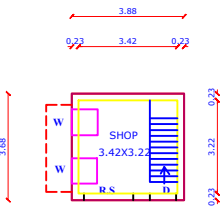
SHOP PLAN
