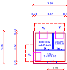
HOUSE PLAN
