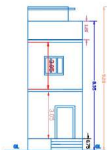
FRONT ELEVATION
