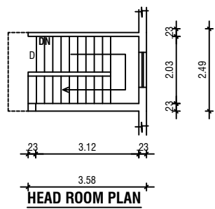
HEAD ROOM PLAN
