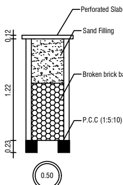
DRAINAGE SOAK PIT DETAILS
