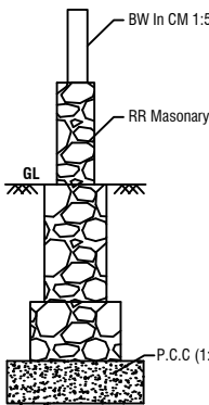
DETAILS OF RR MASONARY
