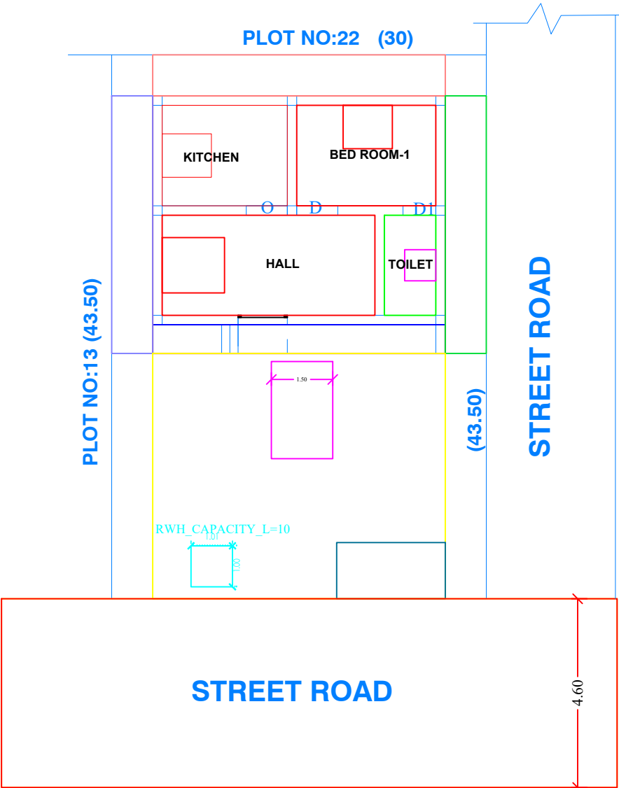
SITE PLAN
