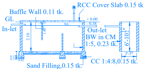
SECTION - SEPTIC TANK
