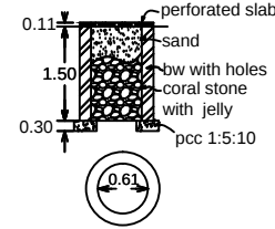
percolation pit
