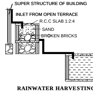
RAINWATER HARVESTING
