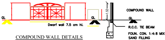
SECTION
