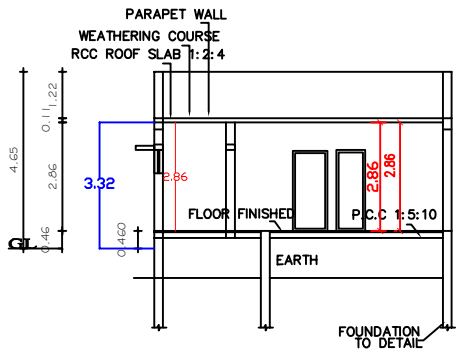
SECTION "A-B"
