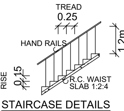
STAIRCASE DETAILS
