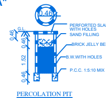
PERCOLATION PIT
