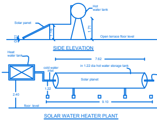
SOLAR WATER HEATER PLANT
