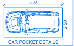
CAR POCKET DETAILS ALL DIMENSIONS ARE IN METRE SCALE: 1:100
