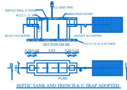
SEPTIC TANK AND TRENCH & U-TRAP ADOPTED
