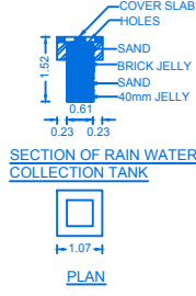
PLAN
