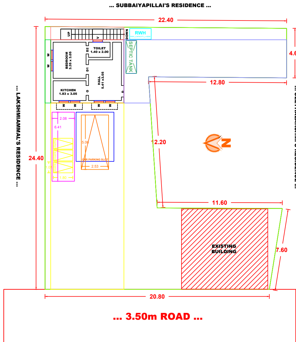
SITE PLAN FOR THE PROPOSAL
