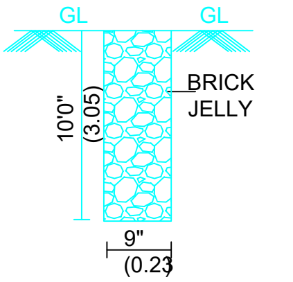
PERCOLATION PIT
