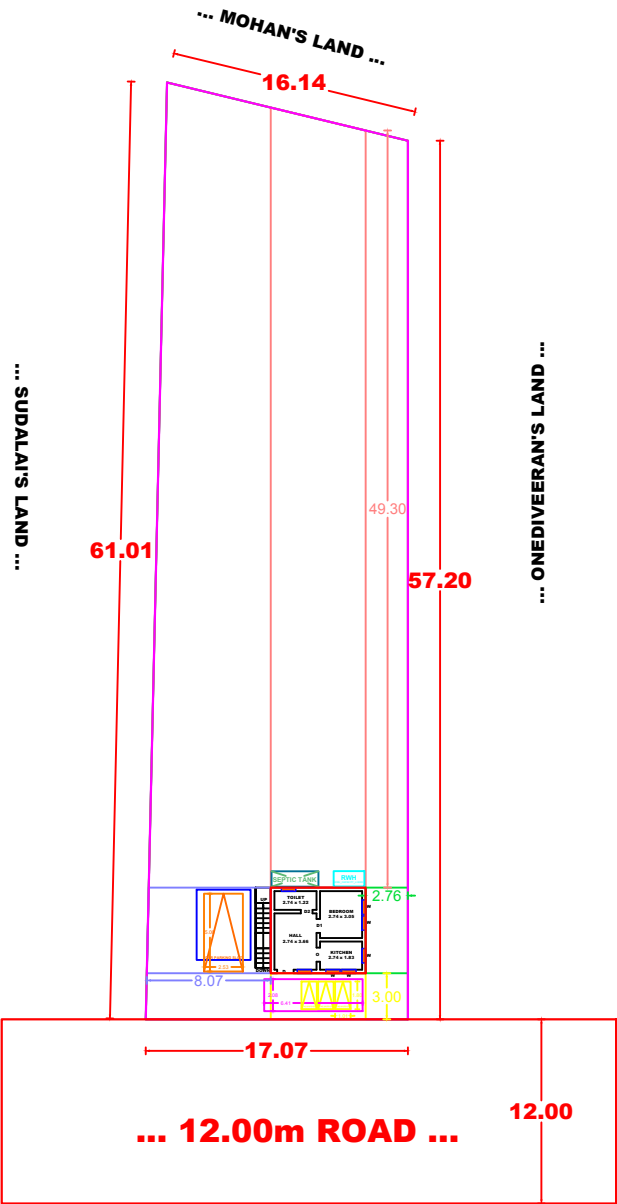
SITE PLAN FOR THE PROPOSAL
