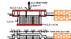
SEPTIC TANK AND TRENCH
