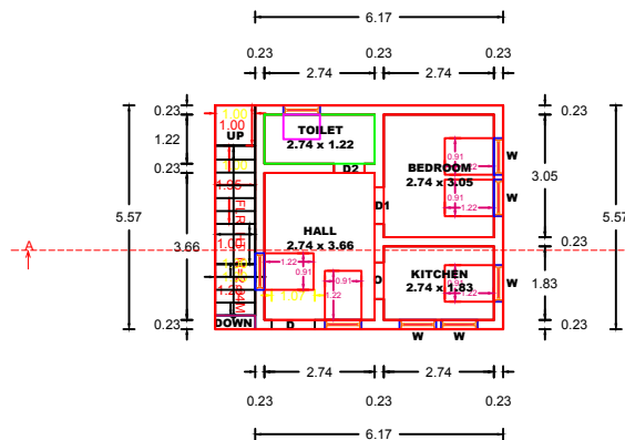
GROUND FLOOR PLAN OF THE PROPOSAL
