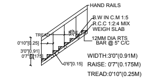
STAIRCASE DETAILS
