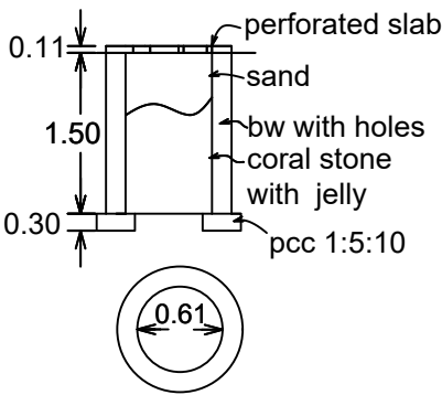
percolation pit
