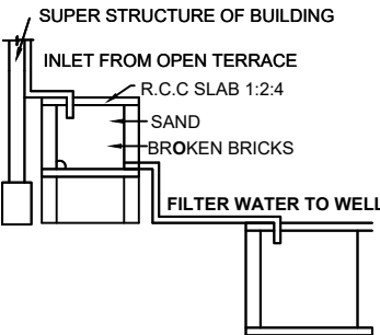
RAINWATER HARVESTING
