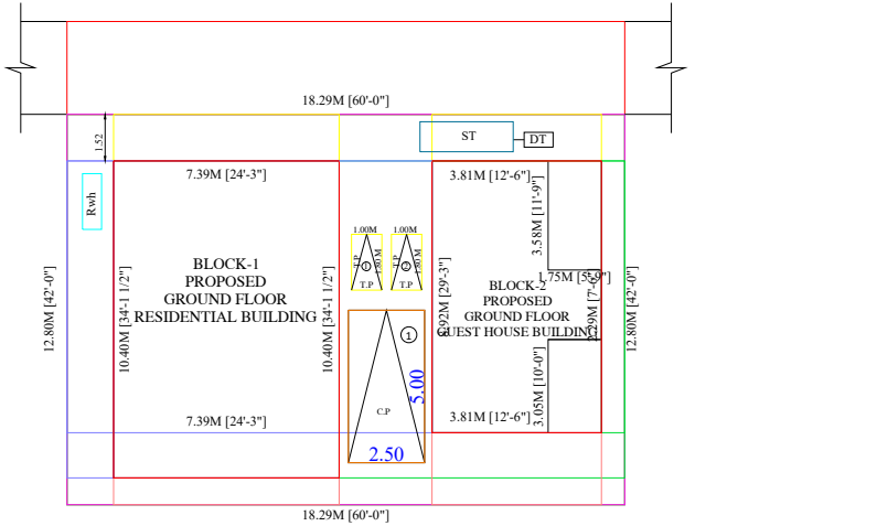
SITE PLAN (MEANT FOR CONTRUCTION)
