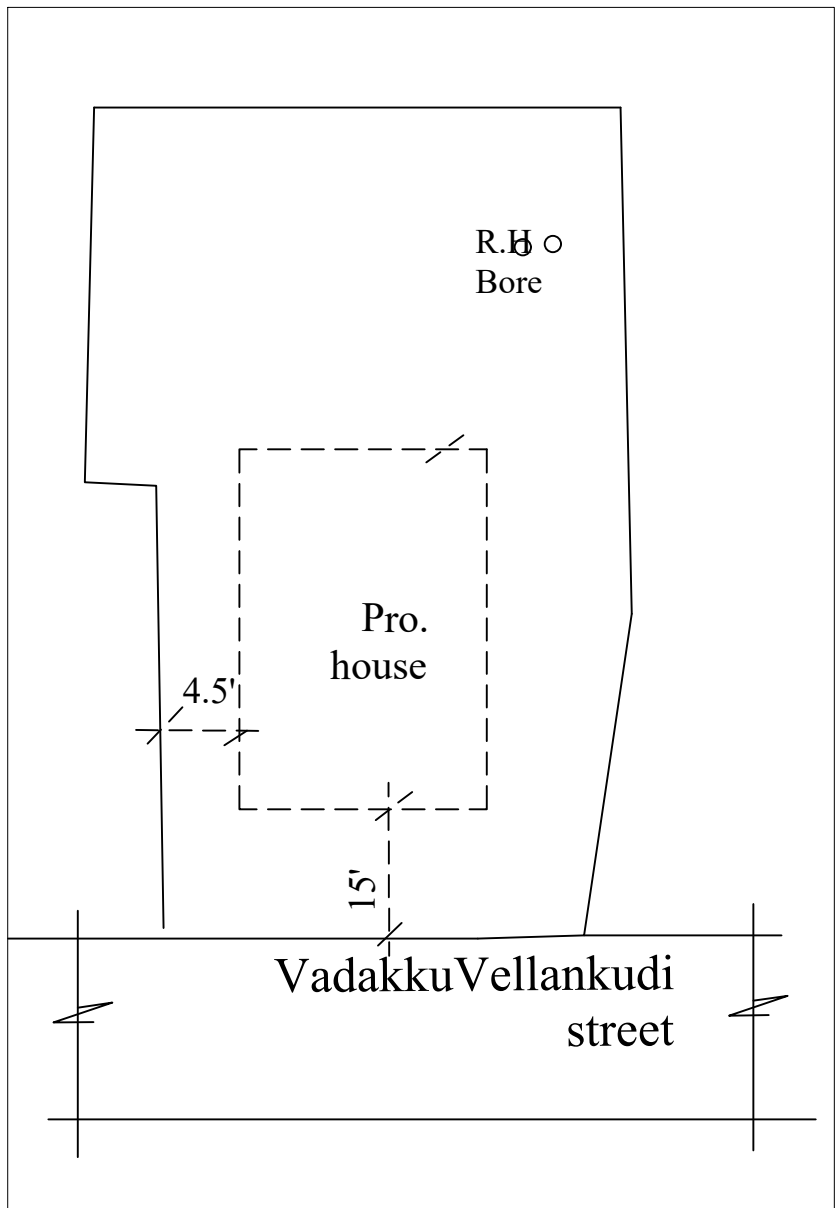
Topo plan scale-1:800
