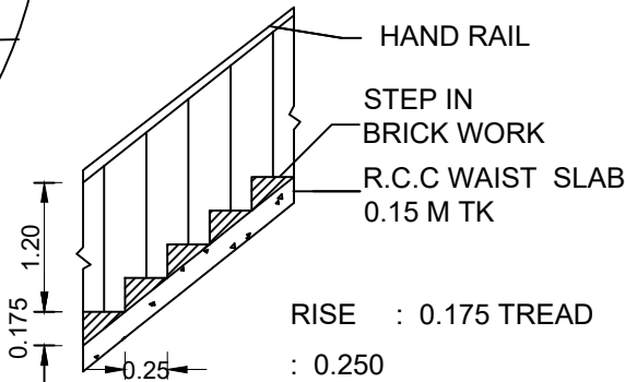
STAIR DETAILS
