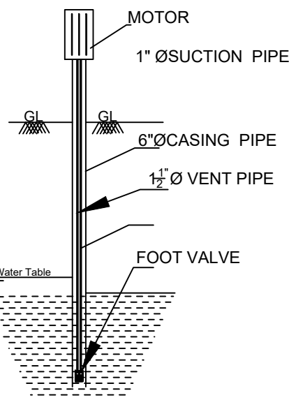
SEC. OF BOREWELL
