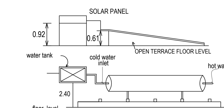
Details of solar water heating system
