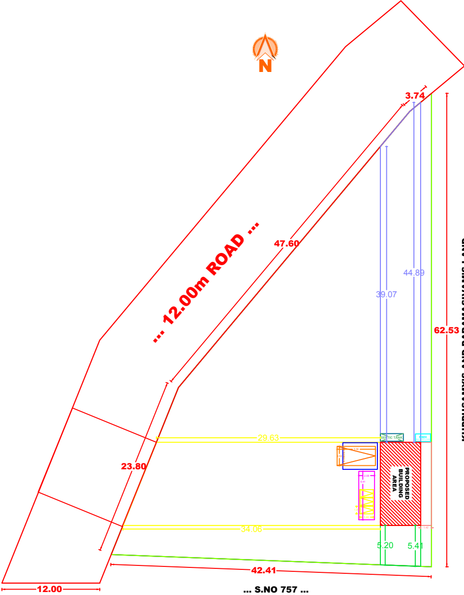
SITE PLAN FOR THE PROPOSAL
