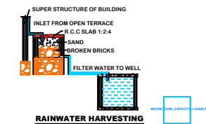
RAINWATER HARVESTING
