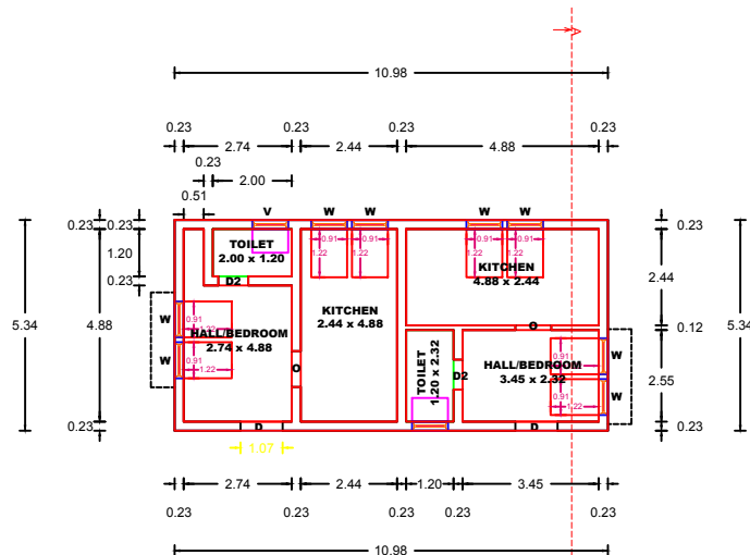
GROUND FLOOR PLAN OF THE PROPOSAL
