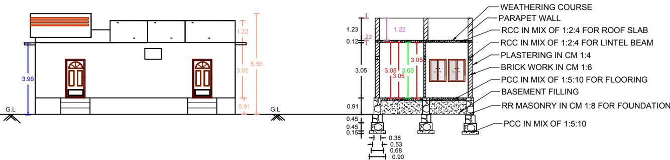
FRONT ELEVATION OF THE PROPOSED BUILDING
