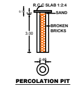
PERCOLATION PIT
