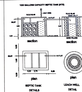
1000 GALLONS CAPACITY SEPTIC TANK (PTE)
