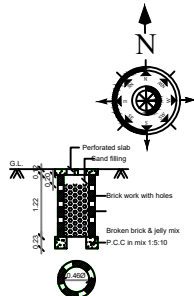
PERCOLATION PIT FOR 30 Sq. m. (Scale:- 1:50)
