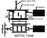
SEPTIC TANK
