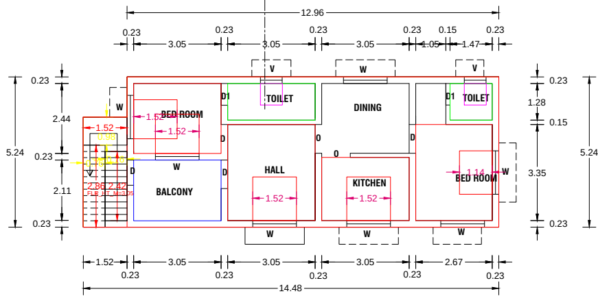
PRO. FIRST FLOOR PLAN
