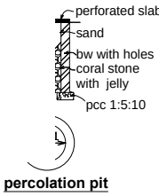
percolation pit
