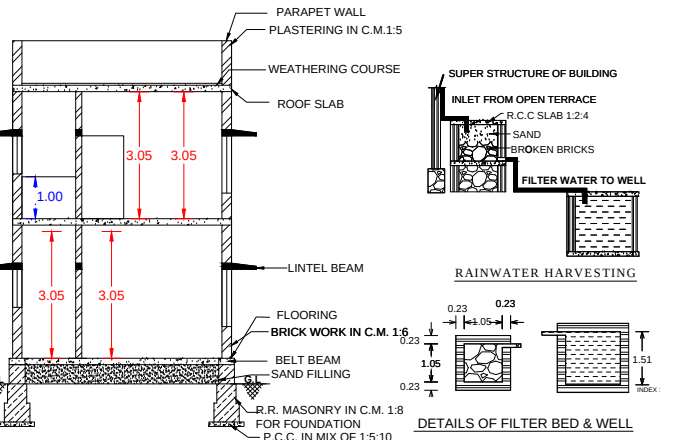
DETAILS OF FILTER BED & WELL
