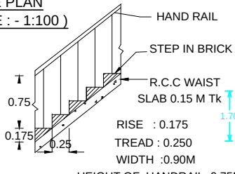
STAIR DETAILS
