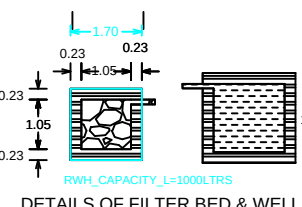
DETAILS OF FILTER BED & WELL
