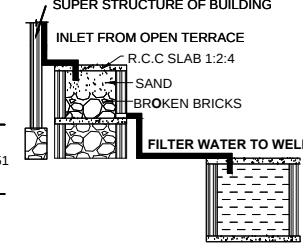
RAINWATER HARVESTING
