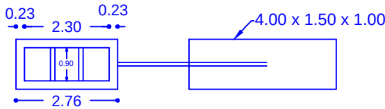
PLAN OF SEPTIC TANK & DISPERSION TRENCH
