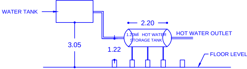
SOLAR WATER HEATING SYSTEM SWHS DETAILS
