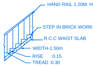
STAIR DETAIL
