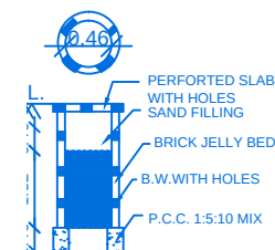
PERCOLATION PIT
