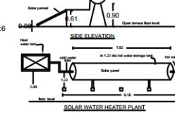
SIDE ELEVATION
